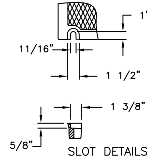
SLOT DETAILS
