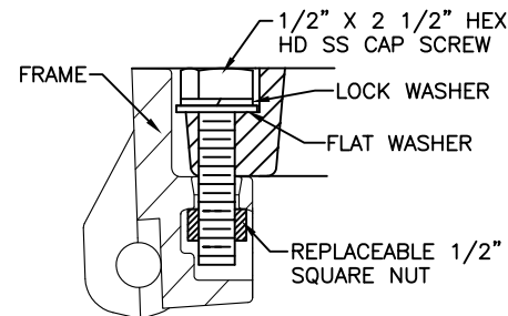
BOLT DETAIL
